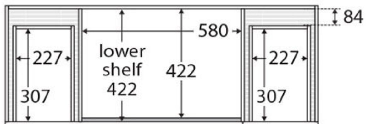
TOP VIEW: SHELF AREA & DRAWER AREA
