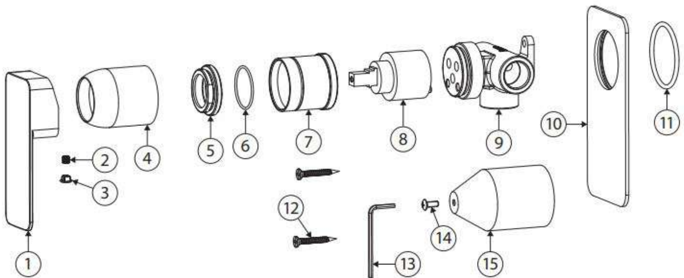
Drawing shown with Tono Wall Mixer Handle (233100) and Large Square Plate (233009)
