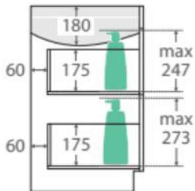
SIDE VIEW: RECESS & DRAWER STORAGE
