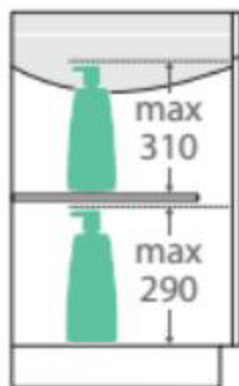
SIDE VIEW: SHELF STORAGE
