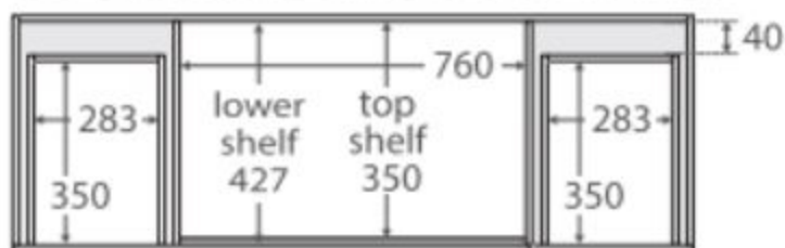
TOP VIEW: SHELF AREA & DRAWER AREA
