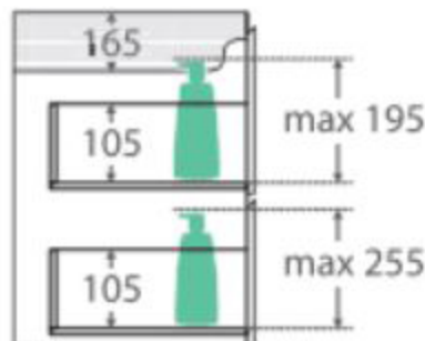
SIDE VIEW: RECESS & DRAWER STORAGE
