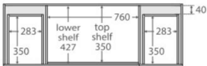
TOP VIEW: SHELF AREA & DRAWER AREA
