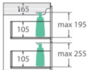
SIDE VIEW: RECESS & DRAWER STORAGE
