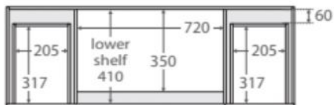
TOP VIEW: SHELF AREA & DRAWER AREA
