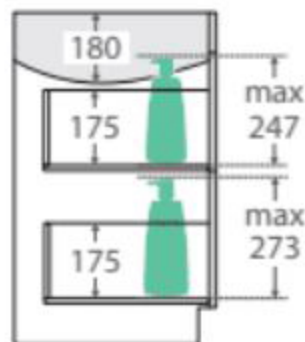
SIDE VIEW: RECESS & DRAWER STORAGE
