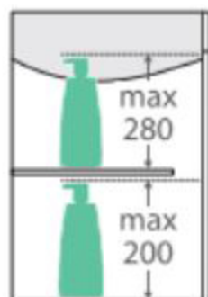
SIDE VIEW: SHELF STORAGE
