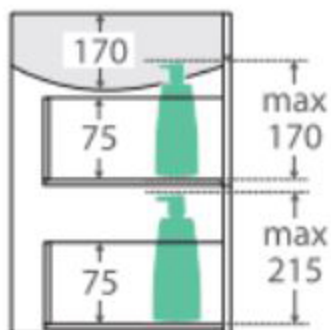
SIDE VIEW: RECESS & DRAWER STORAGE
