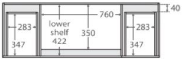
TOP VIEW: SHELF AREA & DRAWER AREA
