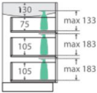
SIDE VIEW: RECESS & DRAWER STORAGE
