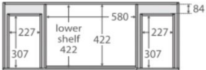
TOP VIEW: SHELF AREA & DRAWER AREA
