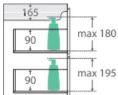
SIDE VIEW: RECESS & DRAWER STORAGE
