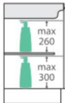
SIDE VIEW: SHELF STORAGE
