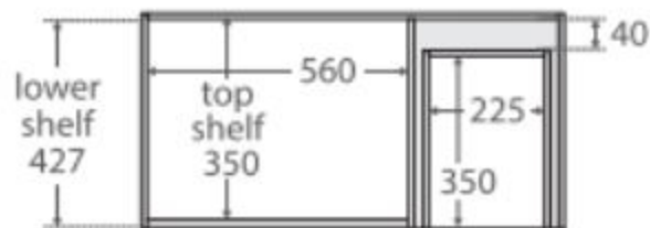
TOP VIEW: SHELF AREA & DRAWER AREA
