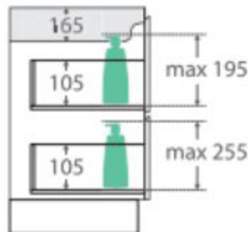
SIDE VIEW: RECESS & DRAWER STORAGE
