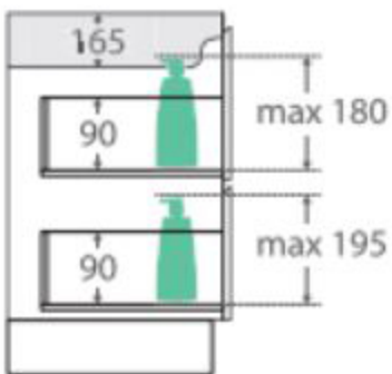
SIDE VIEW: RECESS & DRAWER STORAGE
