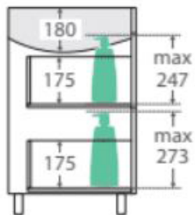
SIDE VIEW: RECESS & DRAWER STORAGE
