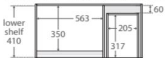
TOP VIEW: SHELF AREA & DRAWER AREA
