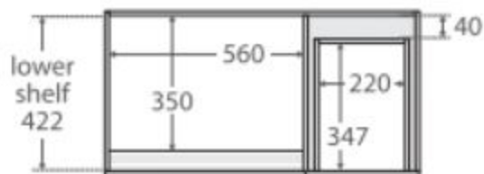
TOP VIEW: SHELF AREA & DRAWER AREA
