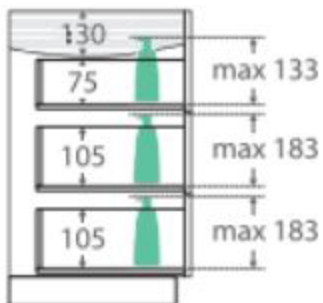
SIDE VIEW: RECESS & DRAWER STORAGE
