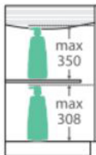
SIDE VIEW: SHELF STORAGE
