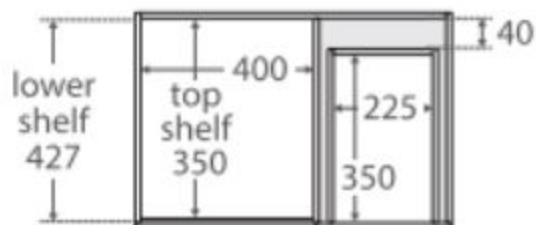
TOP VIEW: SHELF AREA & DRAWER AREA
