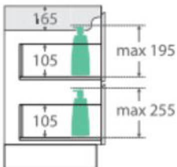
SIDE VIEW: RECESS & DRAWER STORAGE
