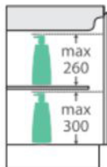
SIDE VIEW: SHELF STORAGE
