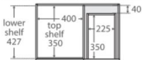
TOP VIEW: SHELF AREA & DRAWER AREA
