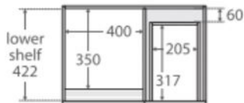
TOP VIEW: SHELF AREA & DRAWER AREA
