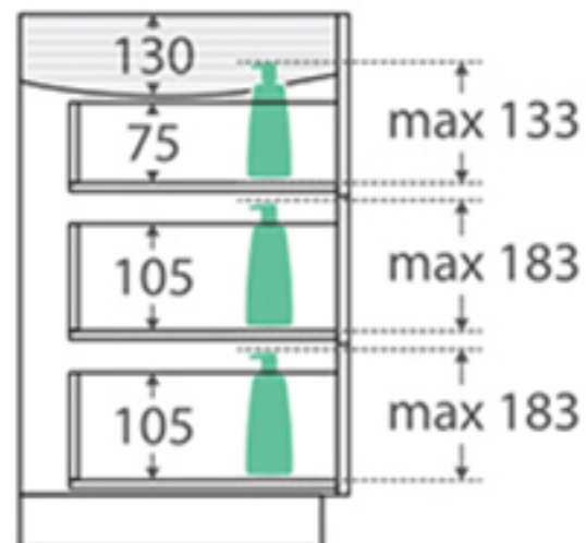
SIDE VIEW: RECESS & DRAWER STORAGE
