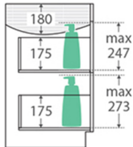
SIDE VIEW: RECESS & DRAWER STORAGE
