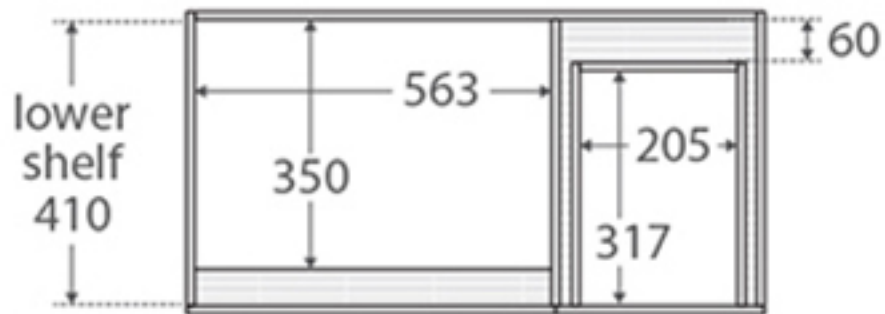
TOP VIEW: SHELF AREA & DRAWER AREA
