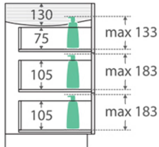
SIDE VIEW: RECESS & DRAWER STORAGE
